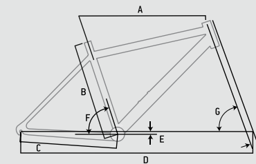
FRAME GEOMETRY CHART
