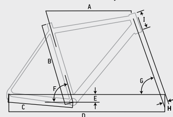
Frame Geometry Chart
