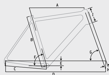
Frame Geometry Chart
