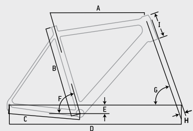
Frame Geometry Chart
