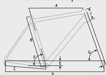
Frame Geometry Chart
